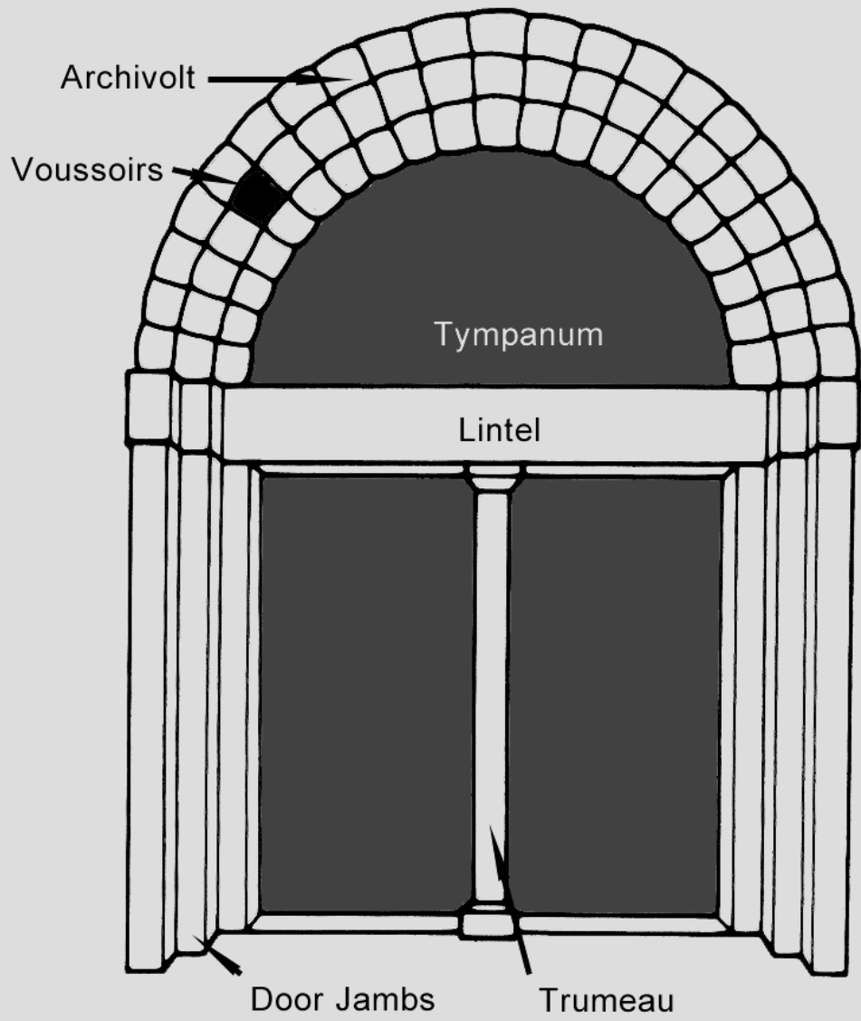
Elements of a Romanesque Portal
