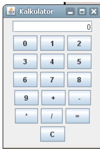
Gambar 1. Tampilan GUI
