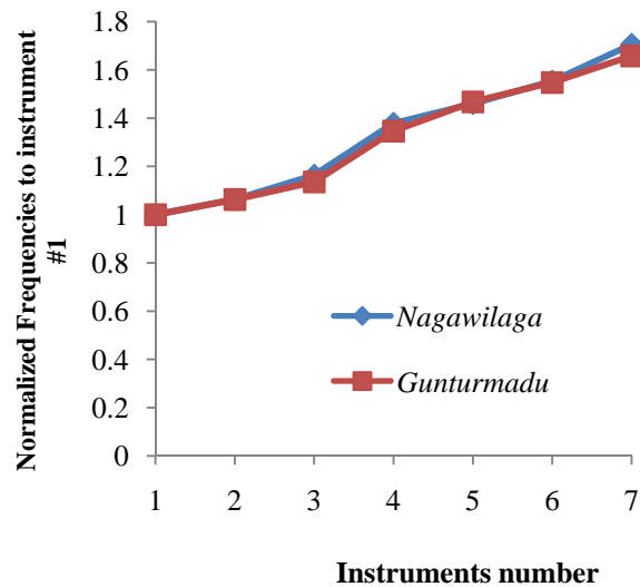
Fig. 4. Comparison of normalized frequencies and the fundamental frequency of instruments number 1 of Saron Ricik , Gamelan Nagawilaga and Gunturmadu
