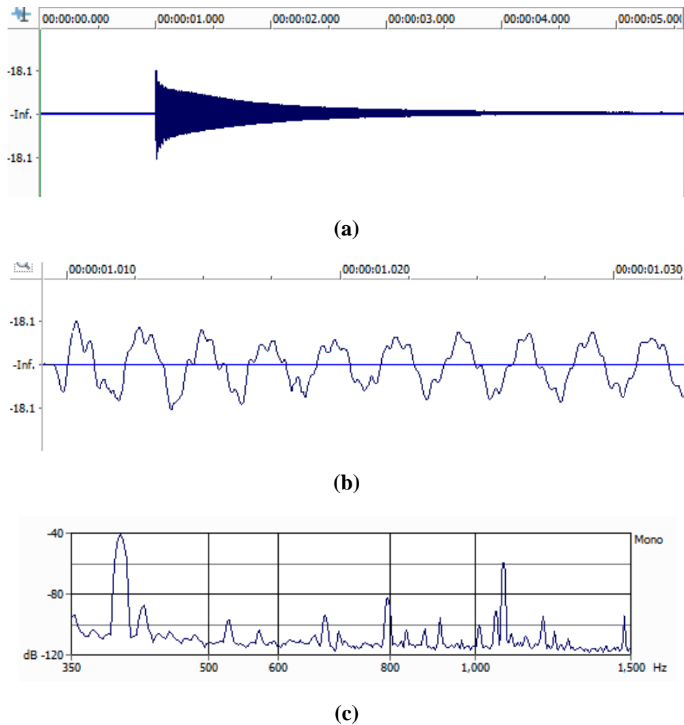
Fig. 1. Instrument #1, Gamelan Saron Ricik Nagawilaga ; (a) waveform as a function of time obtained, (b) magnification of (a), and (c) as a function of the frequency spectrum (Fourier transform of the spectrum (a))
