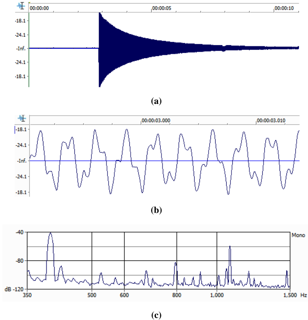
Fig. 2. Instrument #1 Gamelan Saron Ricik Gunturmadu (a) waveform as a function of time obtained instrument 1, (b) magnification of (a), and (c) as a function of the frequency spectrum (Fourier transform of the spectrum (a))
